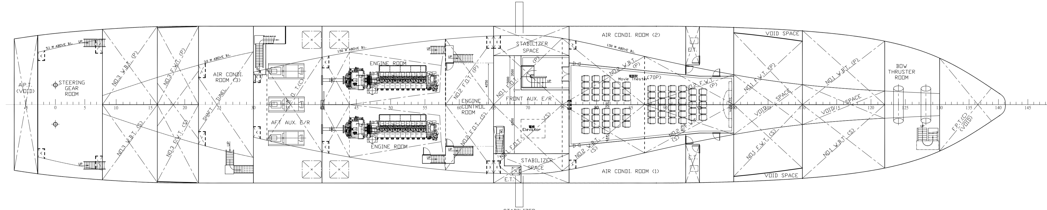
艙頂 TANK TOP 1.50 M ABOVE BL.
